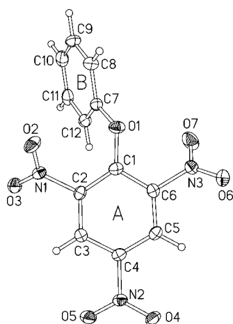
Figure 1. Molecular structure of 4f . Henceforth the atomic displacement ellipsoids are drawn at the 50% probability level.
